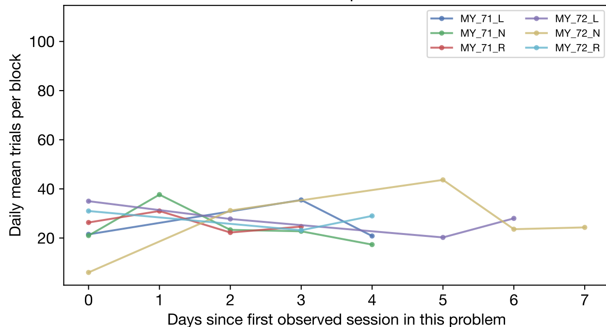
cohort-01 — problem 3
