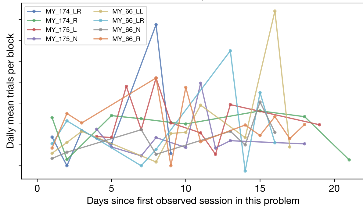
cohort-03 — problem 2
