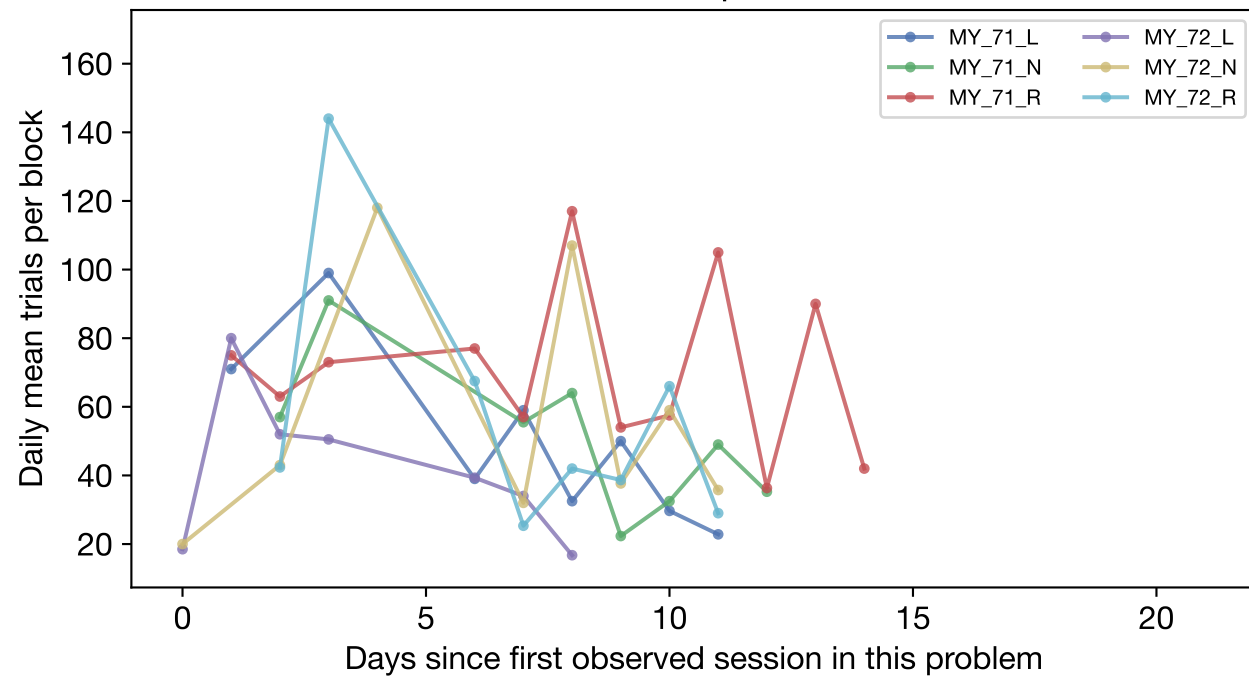
cohort-01 — problem 2
