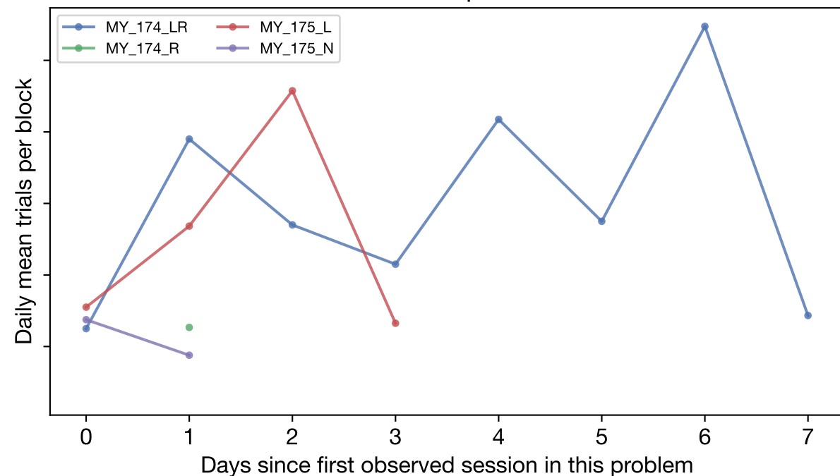
cohort-03 — problem 3
